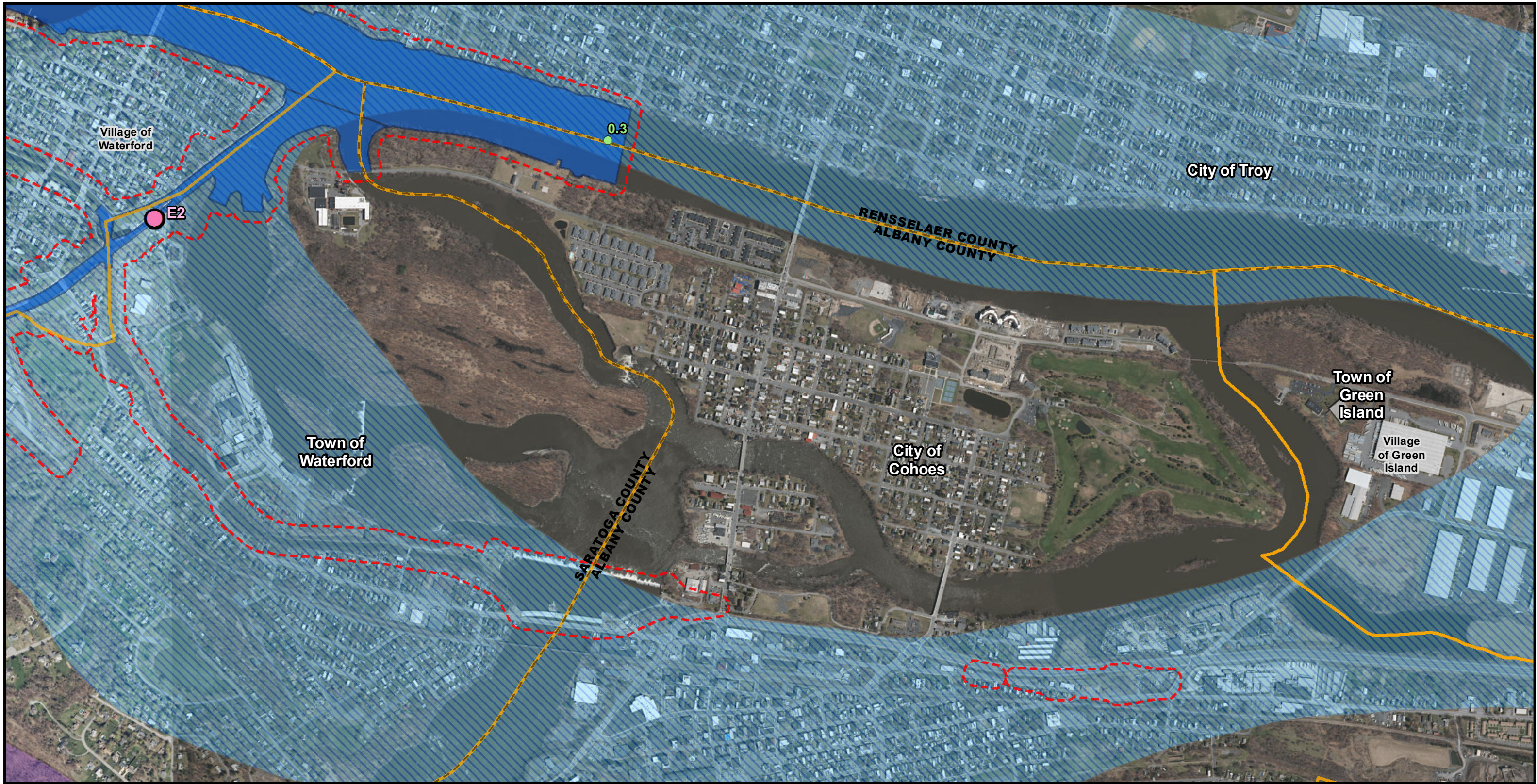
Figure 19F: Aquifers
